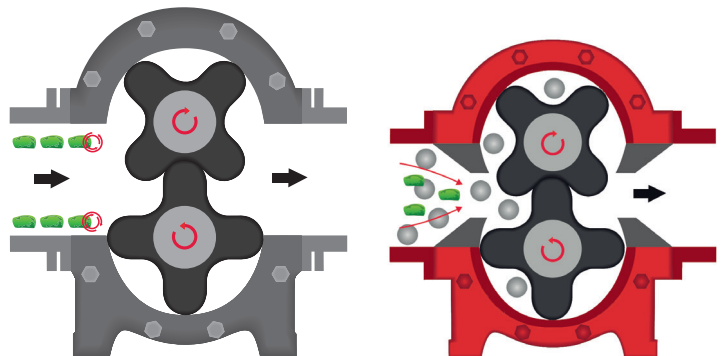
Rotary lobe pump in conventional design
