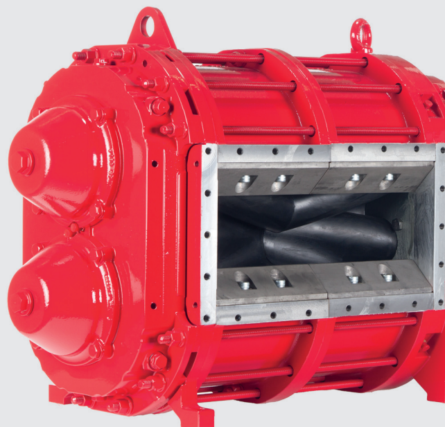
Rotary lobe pump with InjectionSystem
